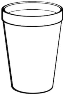
Styrofoam cup
